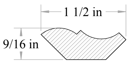
A&M # 5841 9/16" X 1-1/2"
